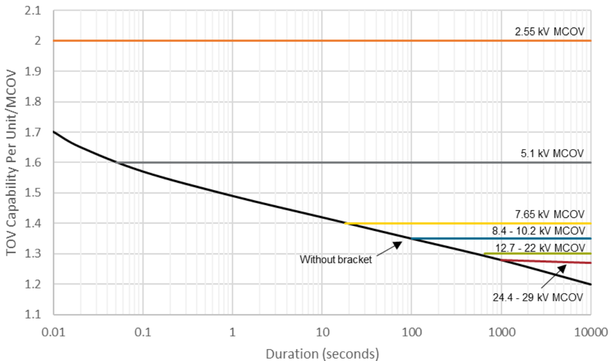
Figure 1: TOV Capability (with and without capacitive ground lead disconnecter bracket)
